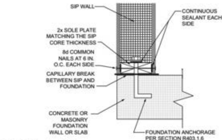
FIGURE R610.5.2 SIP WALL TO CONCRETE SLAB FOR FOUNDATION WALL ATTACHMENT
